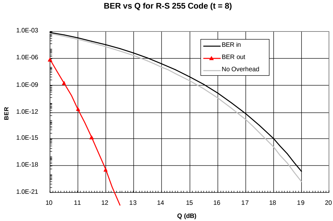
Figure 5 BER vs. Q Factor
