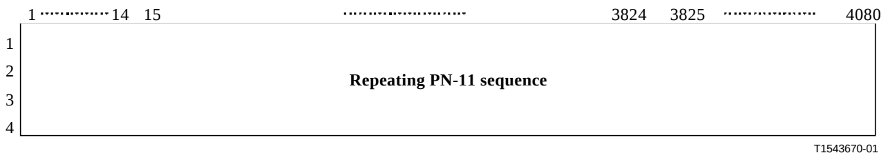
Figure 45 OTUk-AIS (Figure 16-1/G.709)
