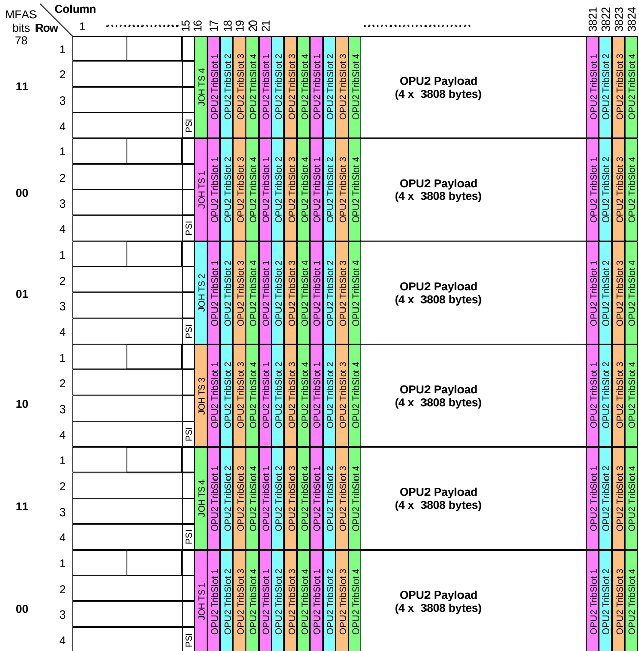
Figure 34 OPU2 tributary slot allocation (Figure 19-1/G.709)
