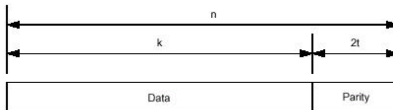
Figure 3 Reed-Solomon Codeword
