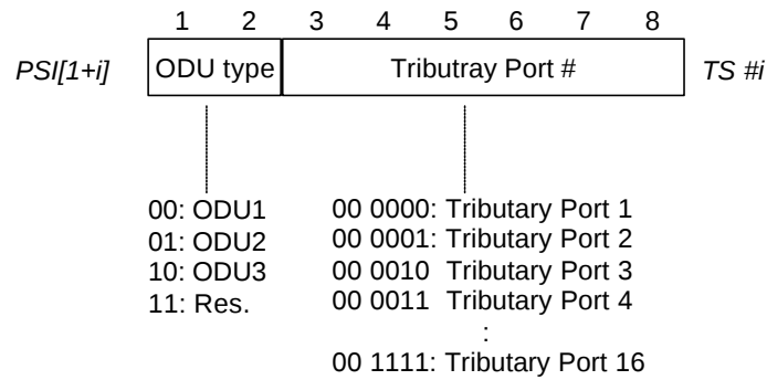
Figure 37 Generic MSI coding (Figure 19-7/G.709)
