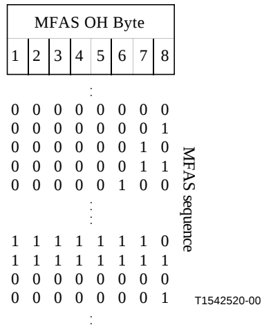
Figure 30 Multiframe alignment signal overhead (Figure 15-8/G.709)
