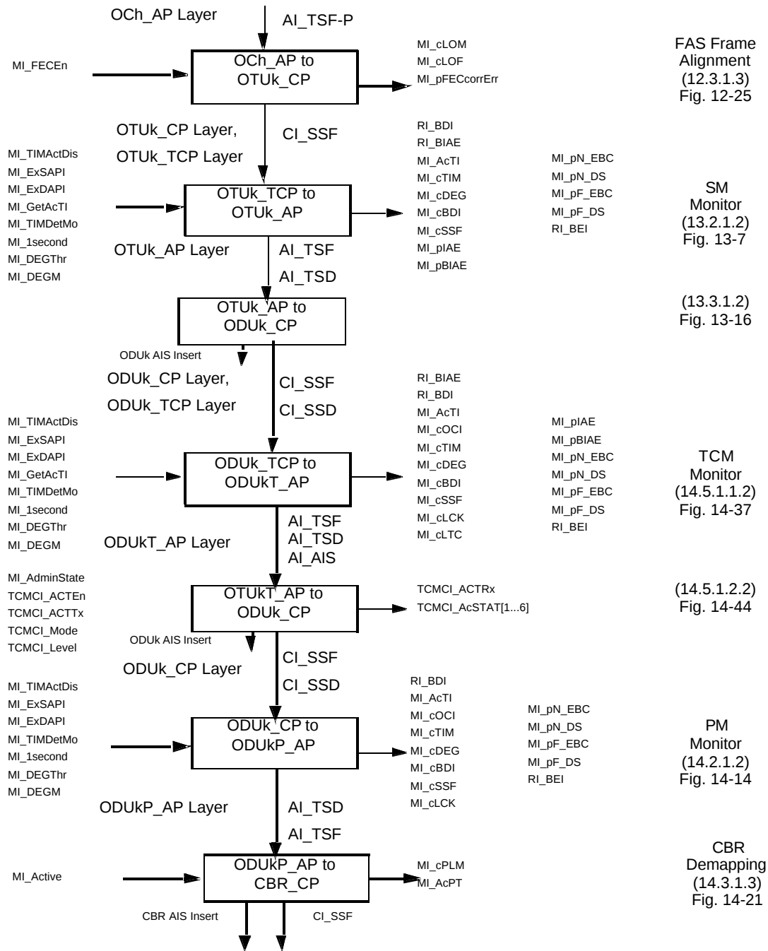
Figure 51 OTN Receive Defects
