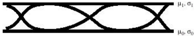
Figure 4 Eye Diagram
