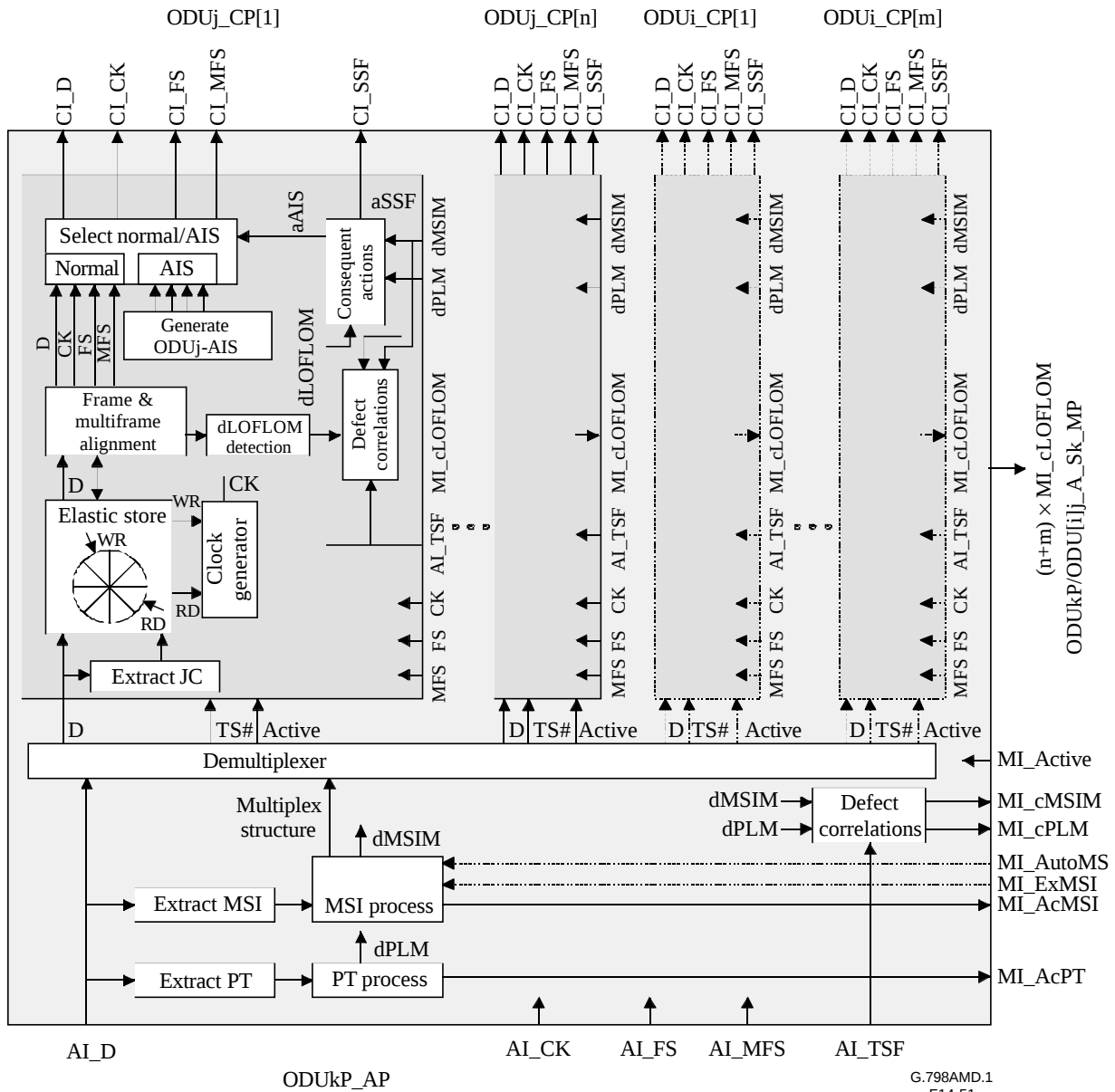
Figure 44 ODUkP/ODU[i]j_A_Sk processes (Figure 14-51/G.798)
