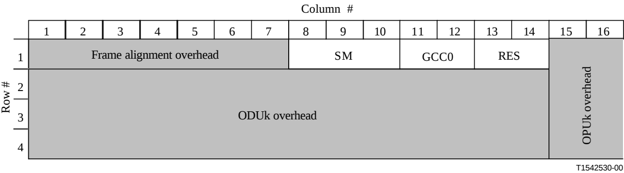
Figure 31 OTUk overhead (Figure 15-9/G.709)
