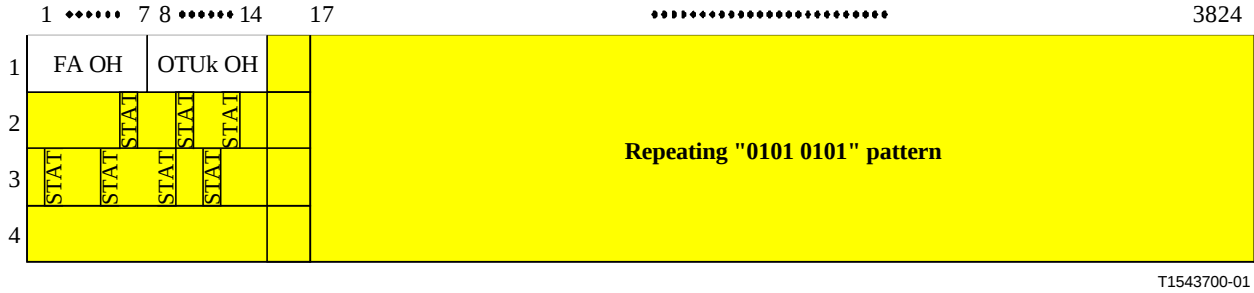
Figure 49 ODUk-LCK (Figure 16-4/G.709)
